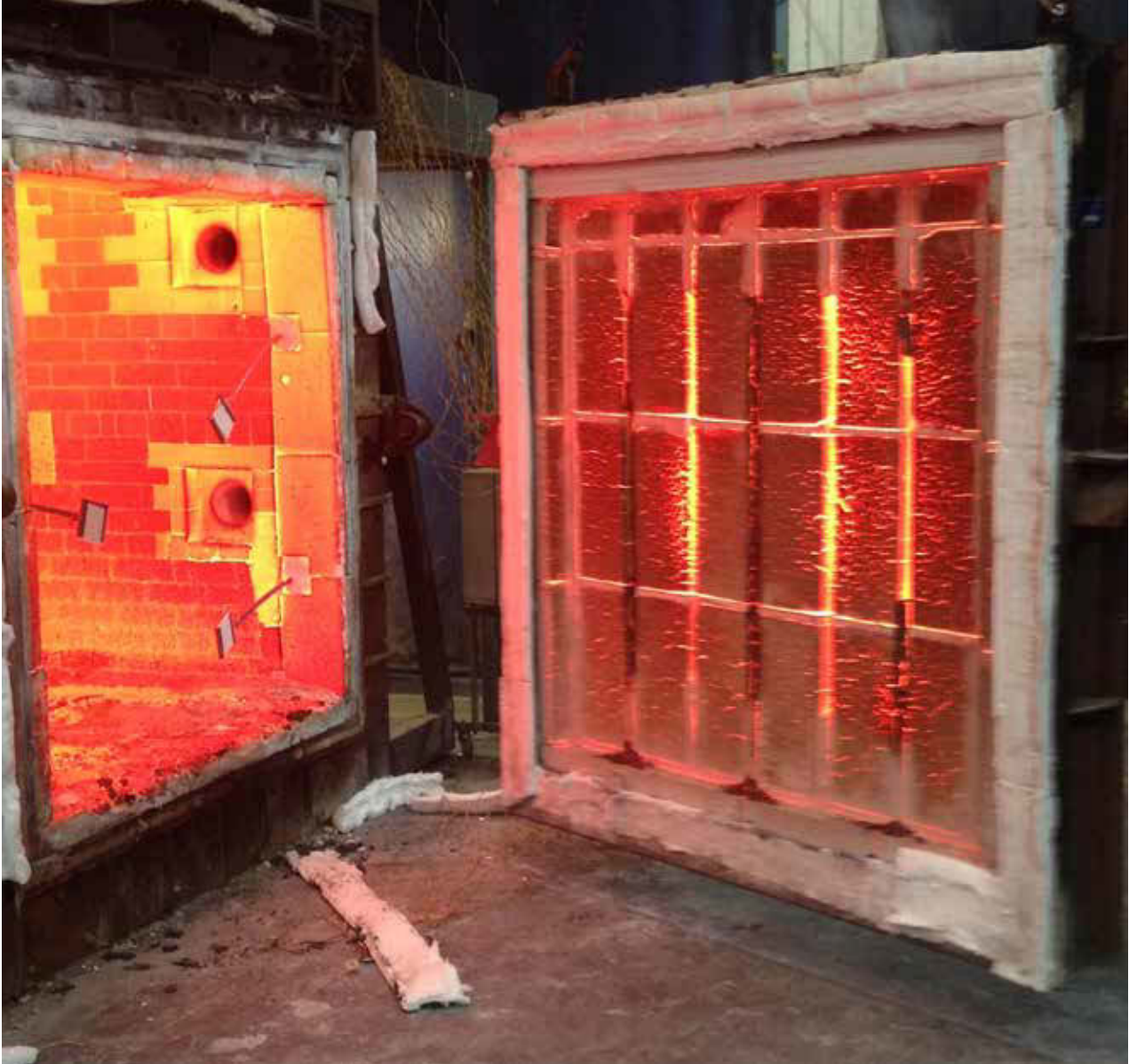
Testing of Sika fire rated sealants at Warrington Fire certification test institute, UK according EN 1366-4
