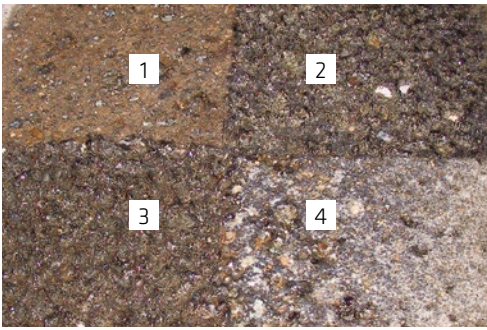
Fig. 8.5.2: Fire exposure trials for concrete containing various aggregates. Surface spalling and sintering, and a range of temperature developments at differing depths can thereby be compared. 1 No spalling, fused surface 2 Limestone; spalling 17 mm, disintegration after cooling + humidity absorption 3 Limestone; spalling 14 mm, disintegration after cooling + humidity absorption 4 Granite; spalling 25 mm, fused surface
