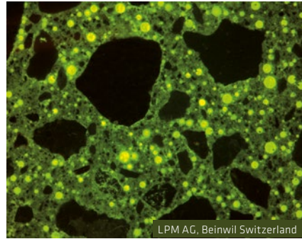
Fig. 8.3.1: Artificially introduced air voids, caused by an air-entrainer, generate space for expansion in the concrete structure to allow for the roughly 10% increase in volume when water freezes to become ice.
