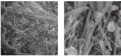
Fig. 8.4.2: Classic form of sulfate attack associated with ettringite or gypsum formation. Flurry of ettringite rods grown in mature cement pastes subjected to external sulfate solutions.
